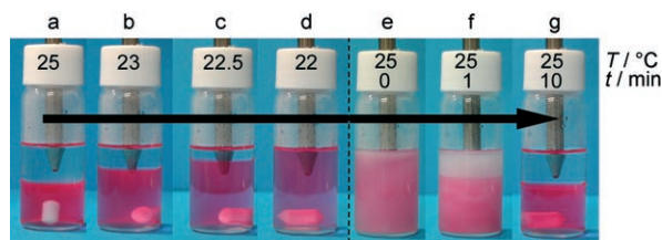
Figure 2. Temperature dependence of the phase behavior of a [\text{P}_{4444}][\text{Tf-Leu}] /water mixture.
